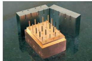
High-efficiency electrical discharge with gate electrode
