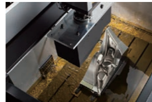
Stable electrical discharge on large 3-dimensional electrode
