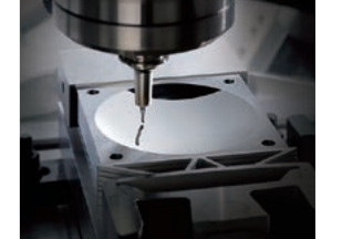
Machining of wide area mirror surface with curvature utilizing linear motors and highly-responsive motion control
